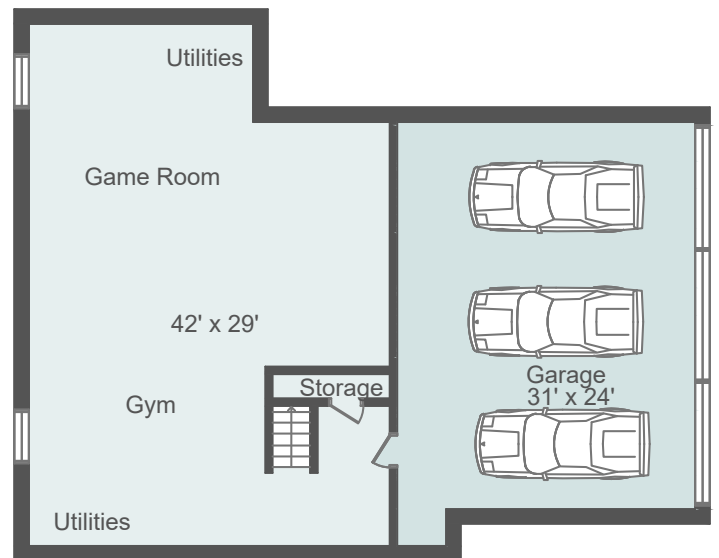
Basement
